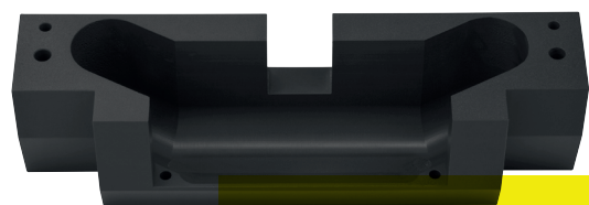
Sensor housing TECASINT 5111: Thermal resistance up to 300 °C. Very good electrical insulation.
